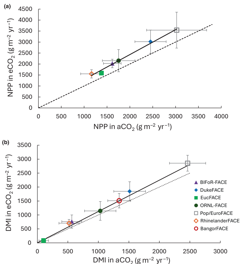
Fig. 2 Forest response to CO 2 enrichment in free-air CO 2 enrichment (FACE) experiments. (a) Net primary productivity (NPP) in eCO 2 (NPPe) vs NPP in aCO 2 (NPPa). The NPPe is adjusted to a common CO 2 enrichment of 41% based on the relationship in Fig. 1. Error bars are SD based on data from each year. The dotted line is the 1 : 1 relationship. The slope of the linear regression equation of NPPe vs NPPa using data from all years at each site (Supporting Information Table S1) is 1.218 \pm 0.011 ( F_{1,39} = 11\,608 , r^2 = 0.997 , P < 0.001 , CI: 1.197–1.245). (b) Similar analysis with aboveground dry matter increment (DMI) yields a slope of 1.182 \pm 0.012 ( F_{1,54} = 9405 , r^2 = 0.994 , P < 0.001 , CI: 1.157–1.206).
