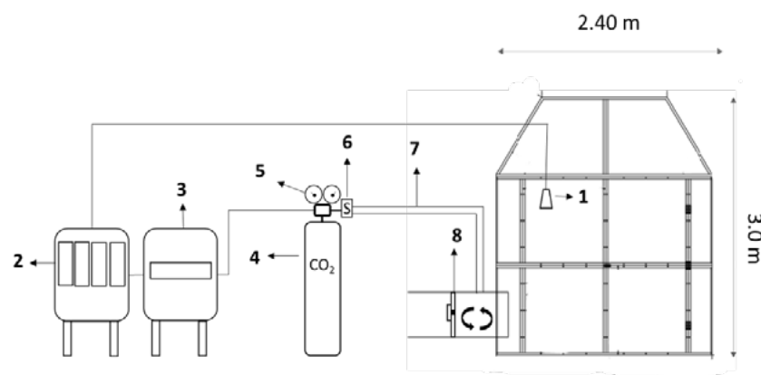
Figure 21. AmazonFACE's Open-Top Chamber Design Structure, Operation Scheme and Its Components. An inlet collector of air samples (1) to analyse \text{CO}_2 concentrations in infrared gas analysers (2). (3) A datalogger stores data and operation software for \text{CO}_2 aspersión. (4) Pressurized \text{CO}_2 cylinder and (5) manometers to control \text{CO}_2 exit pressure. \text{CO}_2 release is controlled by solenoid valves (6), channelled through a rubber tube (7) and mixed with the ambient air through a fan (8) before entering the OTC with \text{eCO}_2 .
