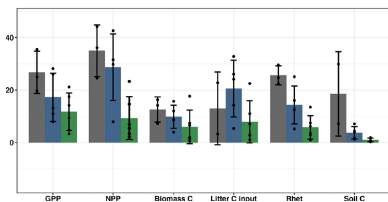
Figure 17. The 15-year modelled response of eCO_2 on productivity (GPP and NPP), biomass C, litterfall, heterotrophic respiration and soil C for dynamic global vegetation models considering C, CN and CNP cycles in the AmazonFACE grid cell. Responses to eCO_2 are the differences between the elevated and ambient model run, shown as mean and s.d. (black lines) per model group, with individual model results as dots.
