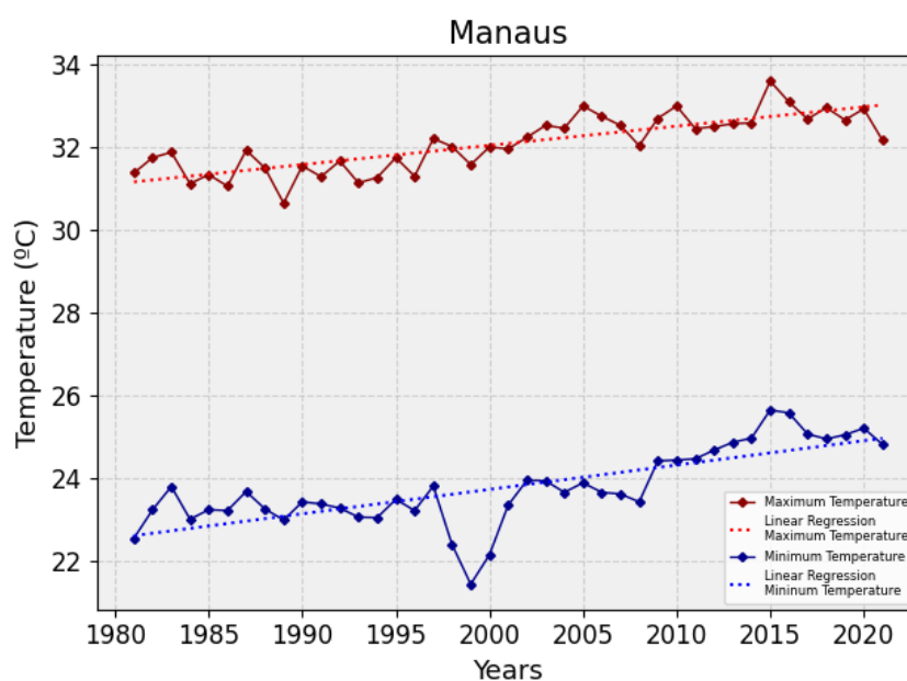
Figure 20. Average Annual Maximum (Red) And Minimum (Blue) temperature (°C) of the municipality of Manaus for the period 1981-2021.
