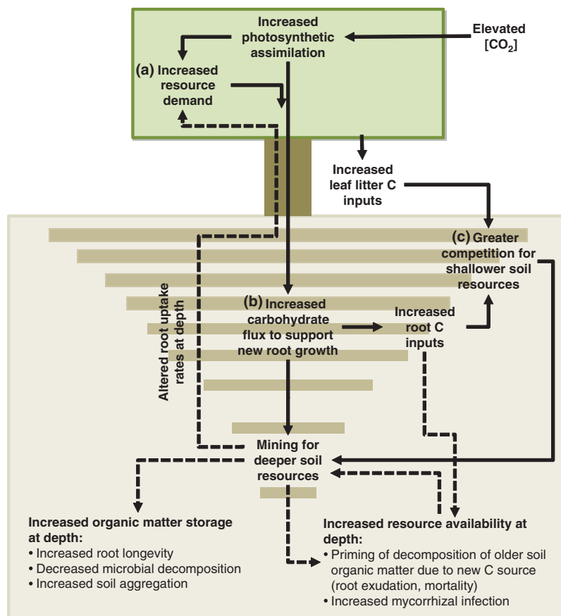
Fig. 1 A conceptual model of the processes leading to deeper rooting distributions under elevated \text{CO}_2 concentration ( [\text{CO}_2] ) (solid lines), and potential feedbacks from the production of deeper roots (dashed lines). Deeper rooting distributions in \text{CO}_2 -enriched forests are probably a result of three interacting factors: (a) increased resource demand by trees, (b) greater carbon (C) available for allocation belowground, and (c) increased competition for scarce resources in shallower soil from microbes or other roots. I have specifically chosen to use the phrase ‘resources’ in the conceptual model rather than ‘nutrients’ to indicate that essential plant resources other than nutrients (e.g. water) may also control rooting distributions under elevated [\text{CO}_2] .
